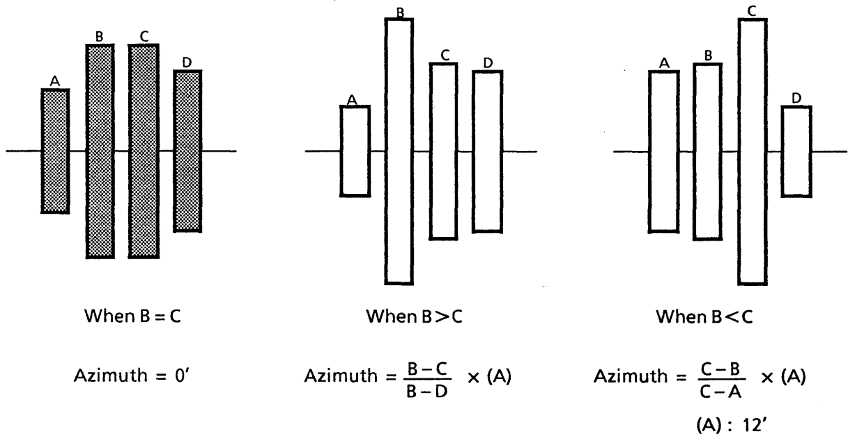
Fig. 9-4 Azimuth Waveforms
